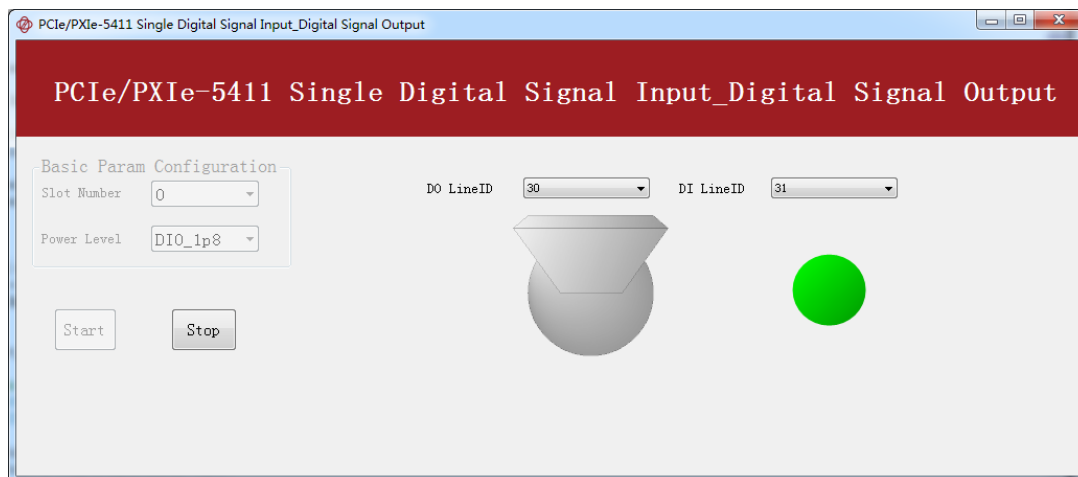
Figure 5 Static DI/DO Loopback Result
