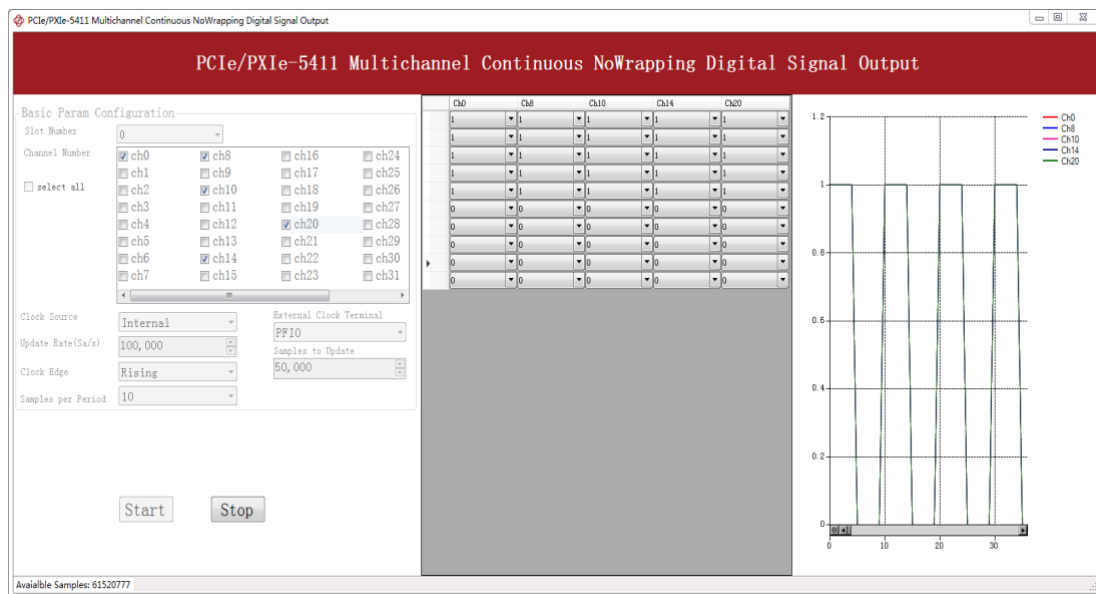
Figure 12 DO Continuous NoWrapping MultiChannel Output Result
