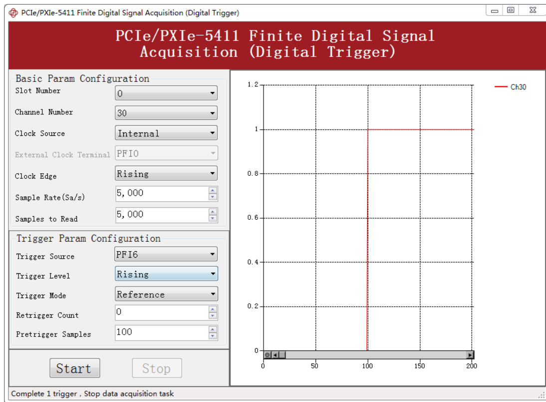
Figure 24 Reference Trigger Acquisition Result
