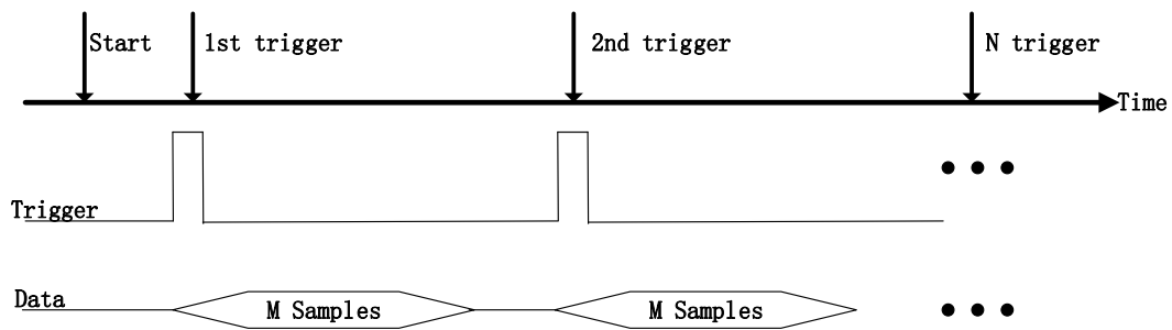
Figure 21 ReTrigger
