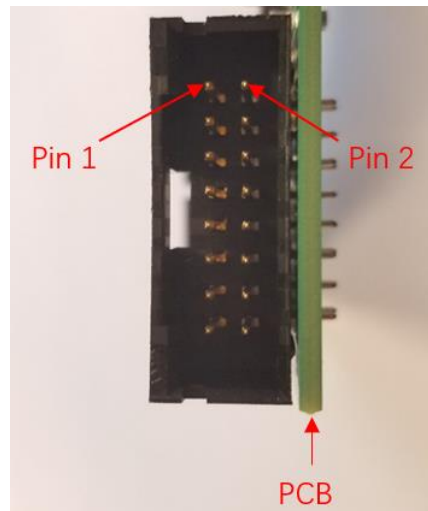
Figure 26 SSI Connector in PCIe-5411
