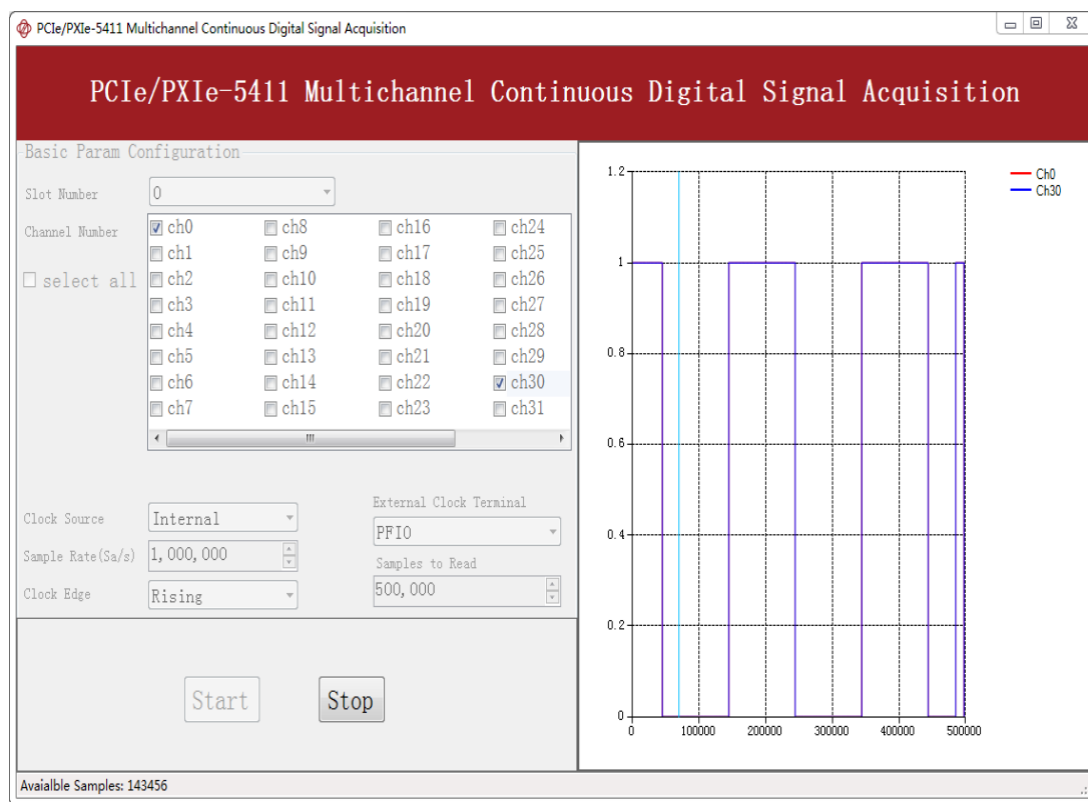
Figure 10 DI Continuous MultiChannels Acquisition Result
