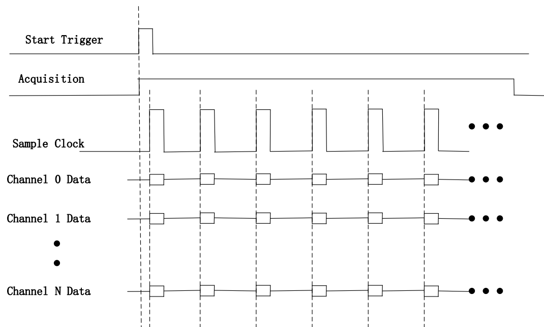
Figure 19 Start Trigger
